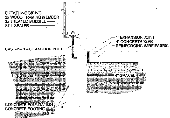
Concrete Slab at Garage Foundation
