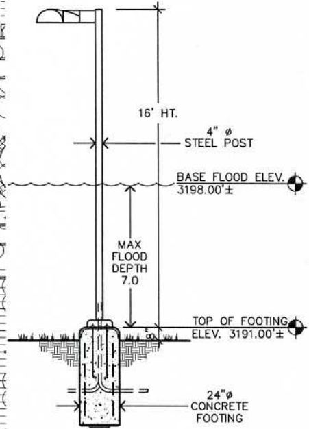
LIGHT POLE ELEVATION SCALE: 1/4"=1'-0"
