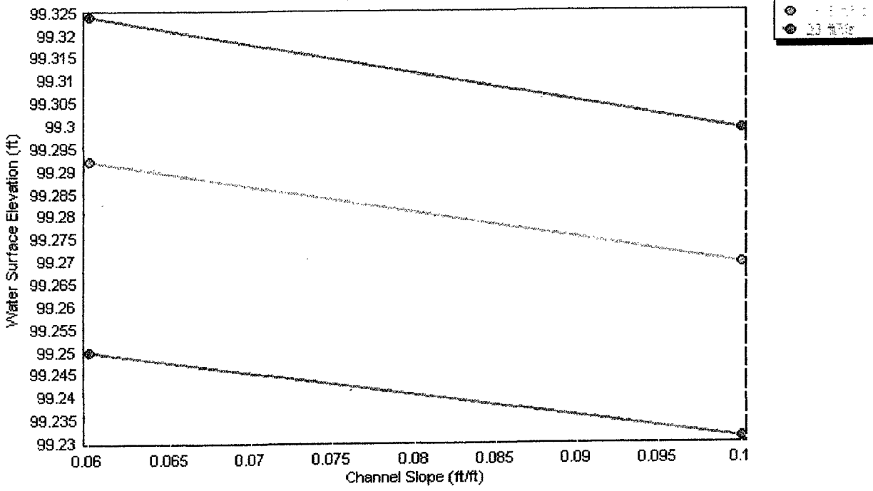
Worksheet: Enchanted Pines Dr / Stumer Road Water Surface Elevation (ft) vs Channel Slope (ft/ft) varying Discharge (ft 3 /s)
