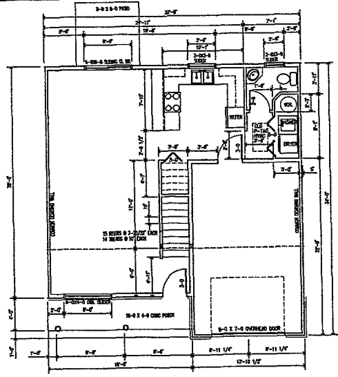
MAIN LEVEL FLOOR PLAN
