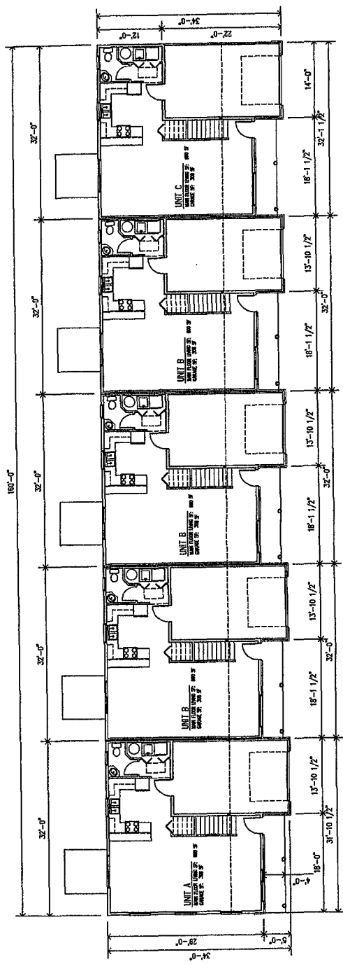
MAIN LEVEL FLOOR PLAN SCALE: 1/8" = 1'-0"
