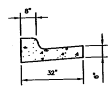
CURB SECTION NOT TO SCALE
