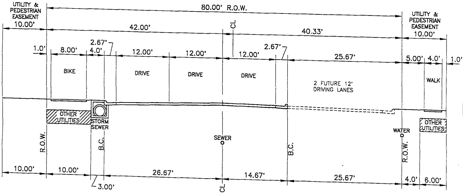
PROPOSED TYPICAL SECTION SCALE: 1:10
