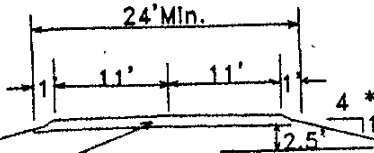
TYPICAL GRAVEL ROAD SECTION
