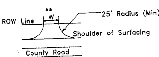
TYPICAL APPROACH DETAIL
