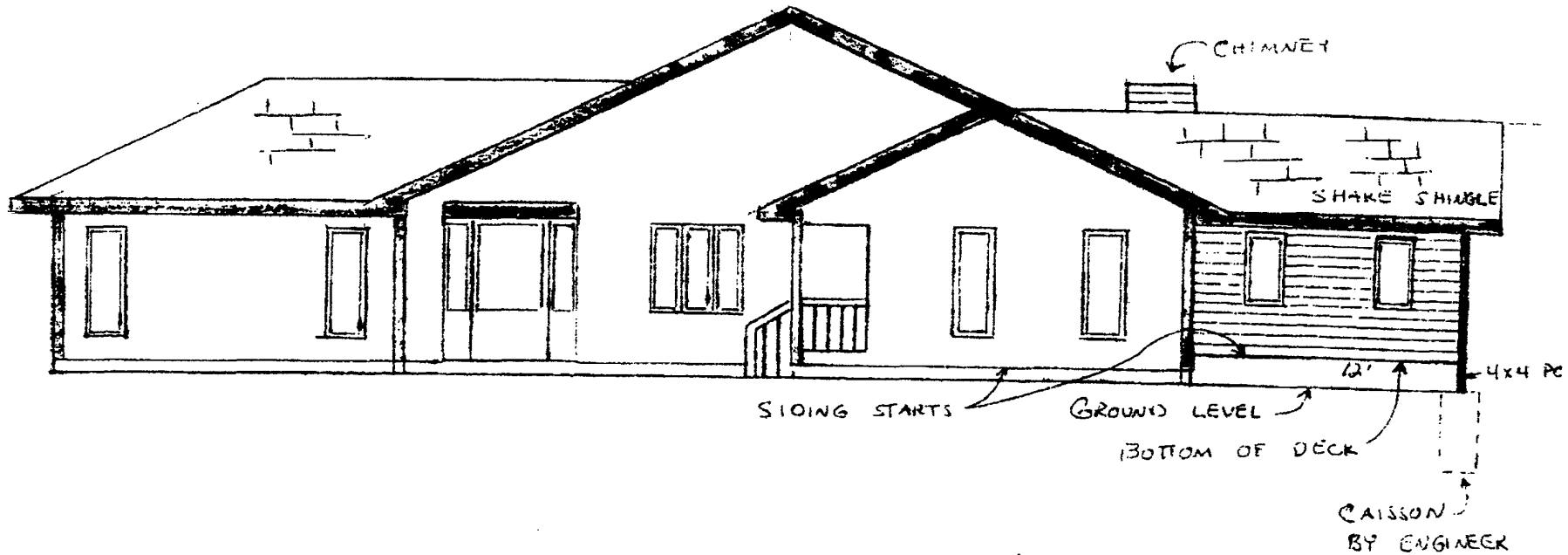
WEST ELEVATION
