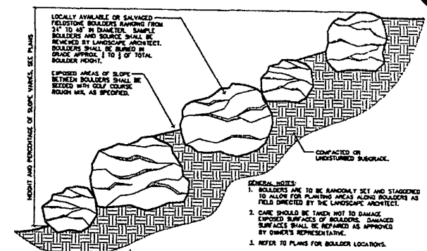
1 SECTION: TYPICAL BOULDER PLACEMENT ON SLOPE NOT TO SCALE
