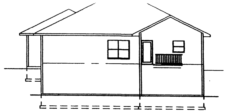
REAR ELEVATION
