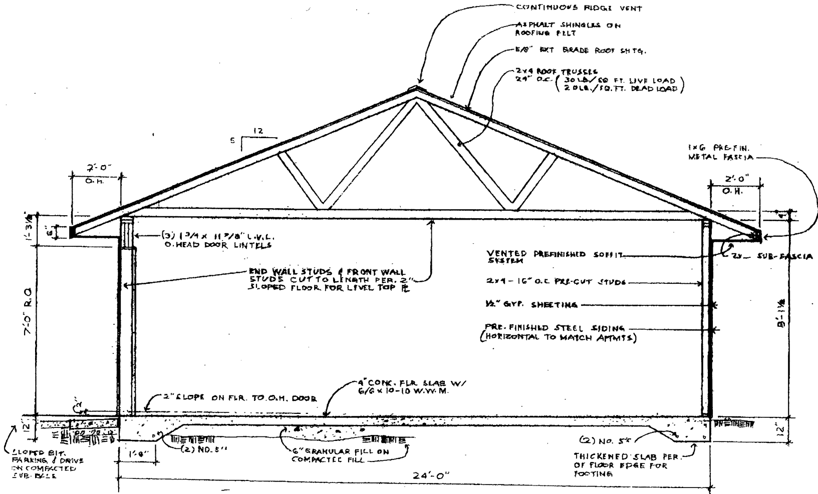
1 SECTION THRU GARAGE AIR
